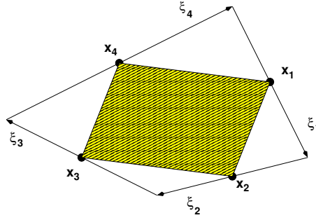
Figure 1. The symplectic area of the quadrilateral, \Delta_4(\xi_1, \xi_2, \xi_3, \xi_4) = \frac{1}{2}(\langle \xi_1, \xi_2 \rangle + \langle \xi_3, \xi_4 \rangle) , determines the phase for the action of the superoperator \hat{T}_{\xi_4} \bullet \hat{T}_{\xi_2}^\dagger and the superoperator \hat{R}_{x_4} \bullet \hat{R}_{x_2} . It is also identified with the phases for the trace of the product of four reflections or four translations that are evaluated in the Appendix.
