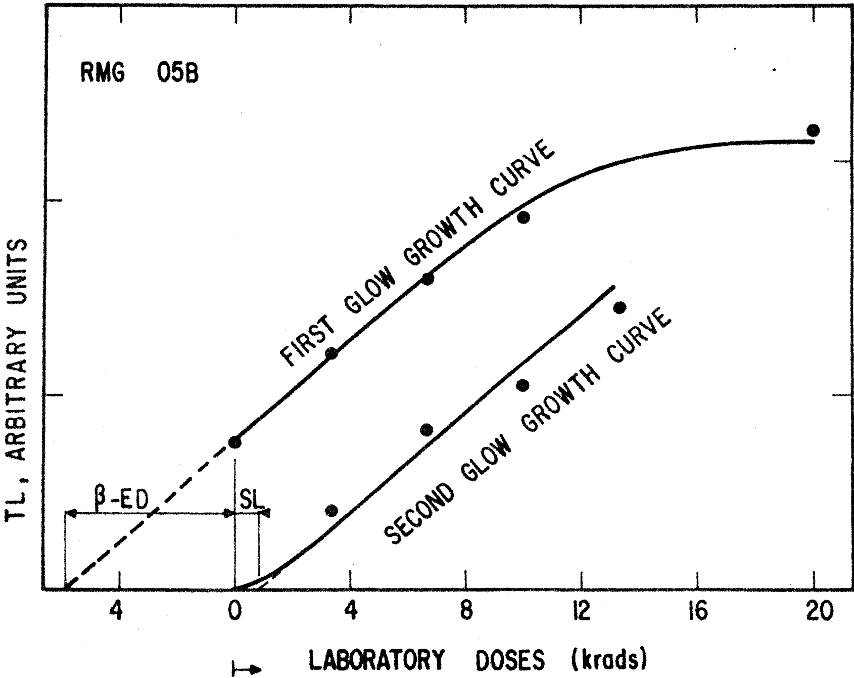
Fig. 8 - TL growth curve for sample RMG 05B for TL emitted at 403C. \beta -ED and SL, respectively \beta - equivalent dose and supralinearity dose correction (uncorrected for solar bleaching).
