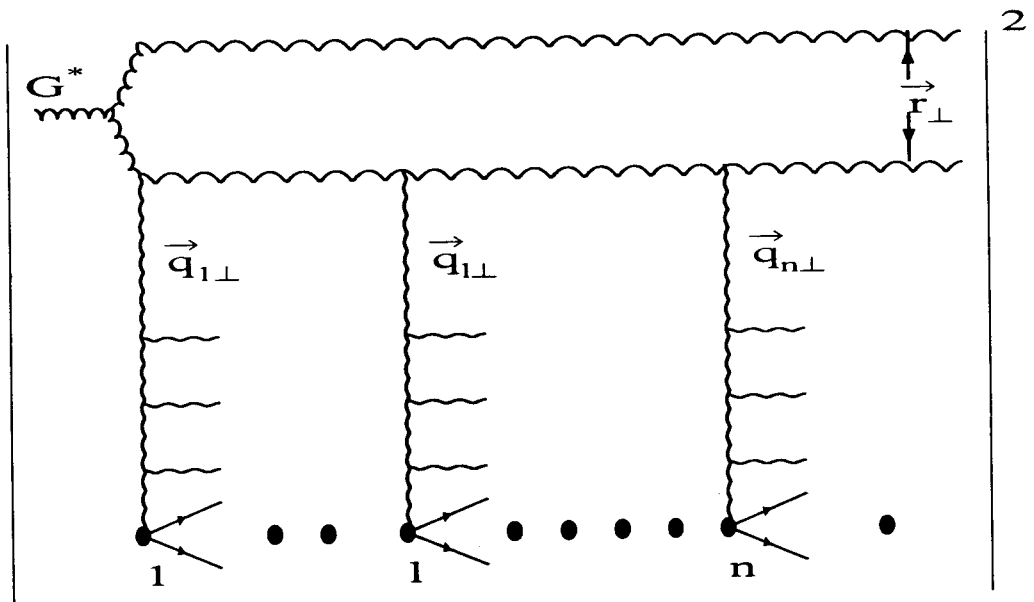
Figure 3: The structure of parton cascade in the Glauber ( Mueller ) formula.
