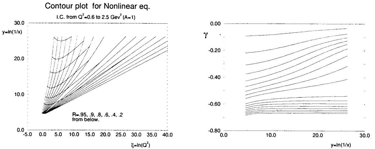
Figure 23: The trajectories and contour plot for the solution of the generalized evolution equation for N . R = \frac{xG(x,Q^2)(\text{generalized equation})}{xG(x,Q^2)(\text{GLAP})} .
