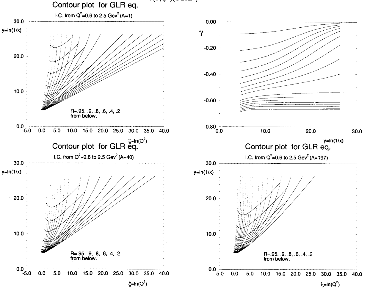
Figure 24: The trajectories and contour plot for the solution of the generalized evolution equation for Ca and Au. R = \frac{xG(x, Q^2)(\text{generalized equation})}{xG(x, Q^2)(GLAP)} .
