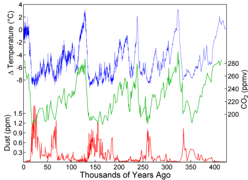
fig 12: Temperature Variations (blue), CO 2 (green) and Dust content (red) in an ice core from the Vostok station in Antarctica over the last 420 000 years. Data from (Petit et al.1999)
