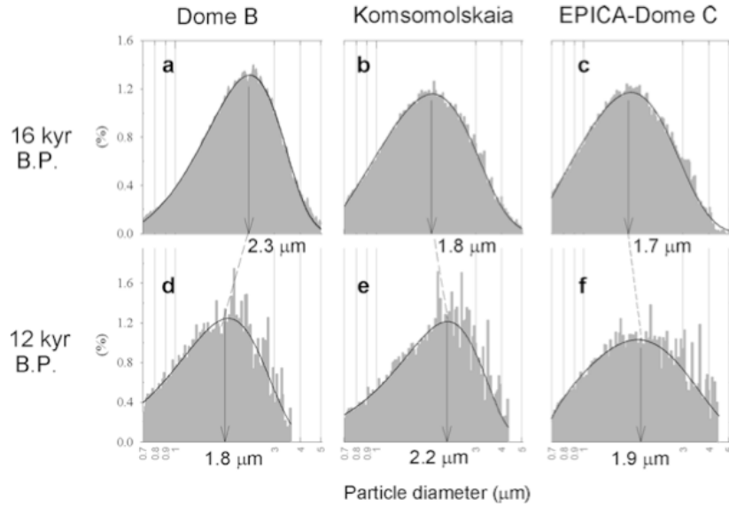
fig 13: Distribution of the small grained dust (radius < 4\mu\text{m} ) from 3 Antarctic sites and two dates. Data from (Delmonte et al.2003).
