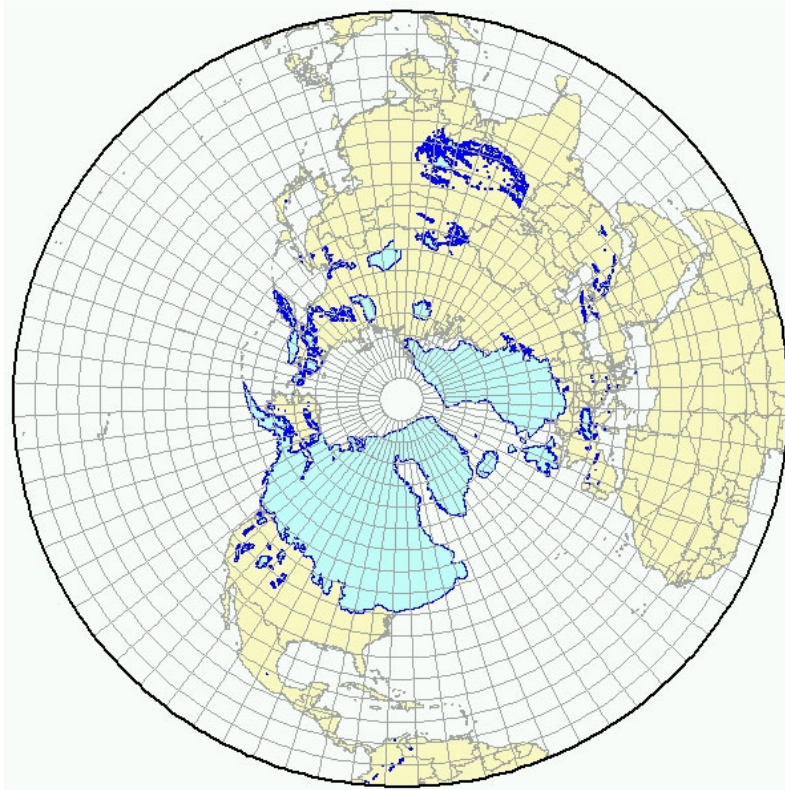
fig 5: The largest glaciation (about 20 000 years ago) was not symmetric with respect to the present position of the North Pole in the Arctic Sea. fig by J, Ehlers. Data from [11]
