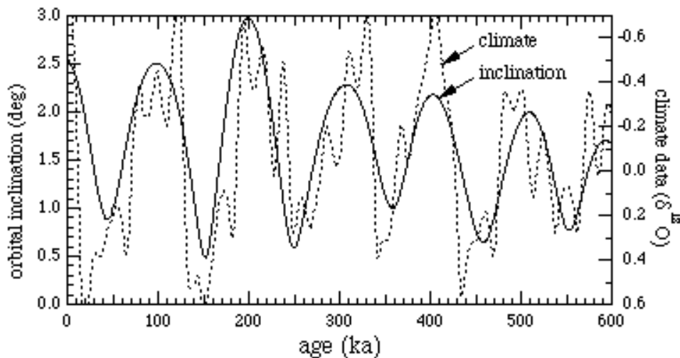
fig 14: The calculated inclination of Earth's orbit (full line) and the isotope variation \delta^{18}\text{O} (dotted line) from [16] for 600 000 years. Figure from [23]
