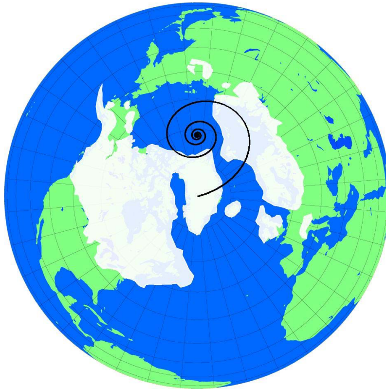
fig 6: Geographic shift of the North Pole: path from Greenland, the assumed center of the largest glaciation, to the present position in the Arctic Sea. One turn of the spiral takes about 400 days (Chandler period). fig from [32]
