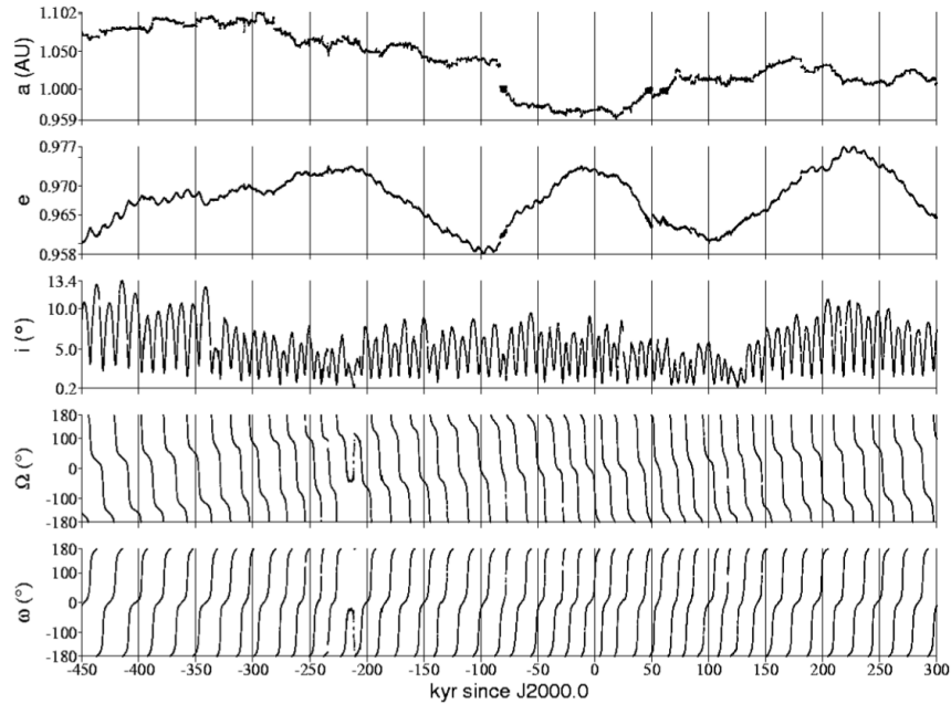
fig 16: Calculated Milankovitch variations of the orbital parameters of Z with assumed mass 0.11M_E . ( a , semi-major axis; e , eccentricity; i , inclination; \Omega , longitude of the perihelion; \omega , argument of the perihelion) over 750 kyr. Note the short cycles of the inclination. Details of the calculation are found in section 2 of [25].
