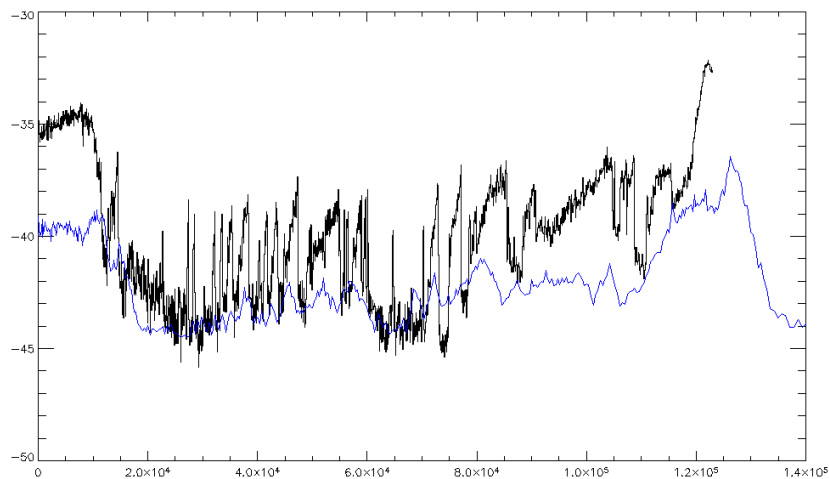
fig 9: Temperatures from Oxygen isotopes in Greenland (black) and Antarctica (blue) between present and 140 000 years before present.
