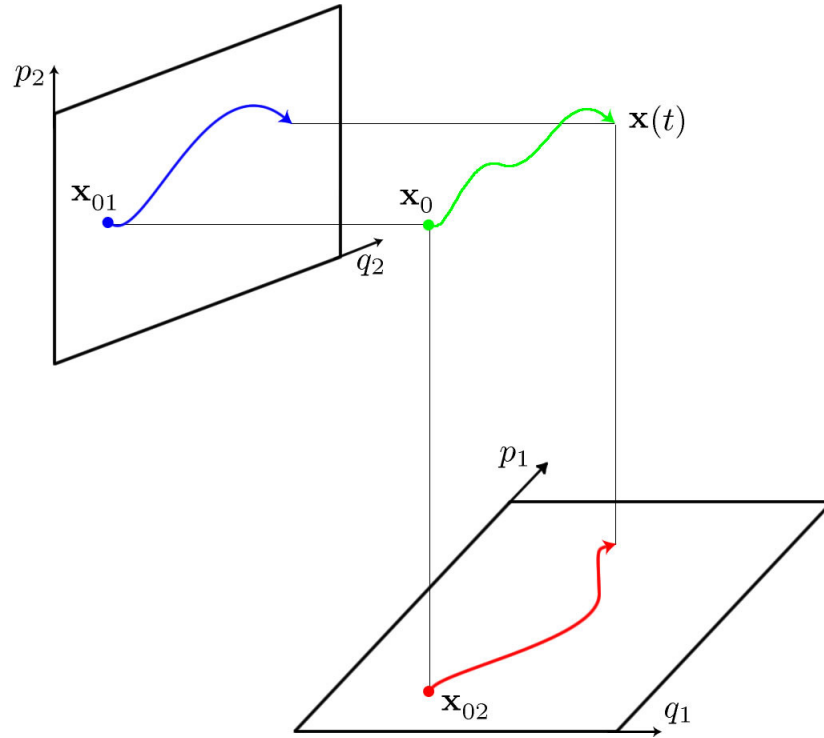
Fig. 1. The classical trajectories, \mathbf{x}_1(t) and \mathbf{x}_2(t) , for each component in its own phase space, are projections of the full trajectory for the entire system.
