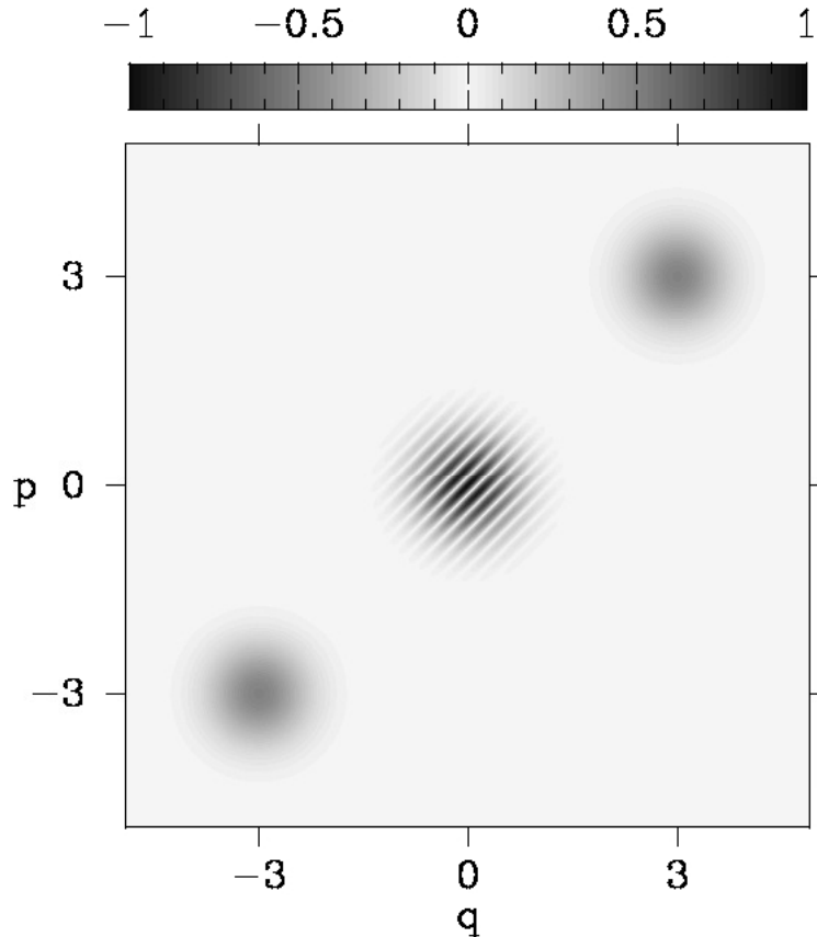
Fig. 6. The Wigner function for the Schrödinger cat state displays a pair of classical Gaussians, one for each coherent state, and a third Gaussian modulated by interference fringes halfway between them. The chord function is a mere rescaling of the Wigner function if the midpoint lies on the origin.
