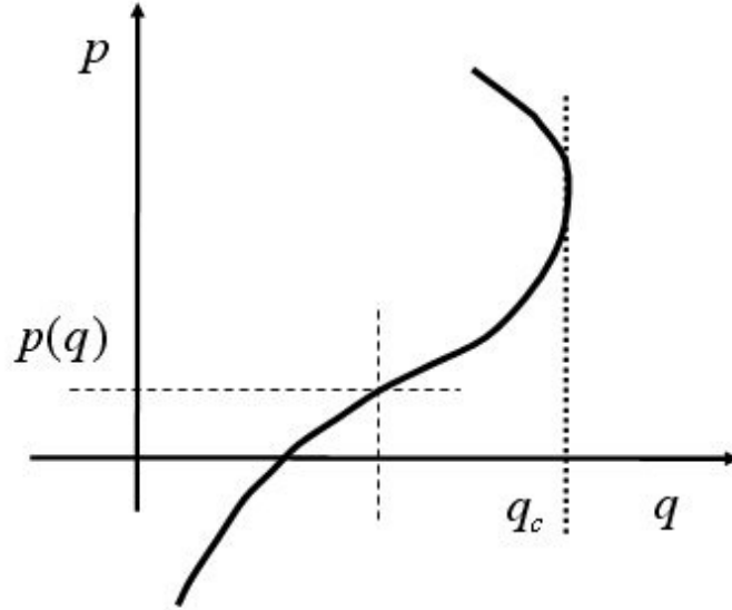
Fig. 2. The caustic of the semiclassical approximation to \langle q|k\rangle lies in the neighbourhood of the point q_c , where the tangent to the classical curve is vertical. The projection of this region onto the p axis is nonsingular, leading to a good semiclassical approximation for \langle p|k\rangle .
