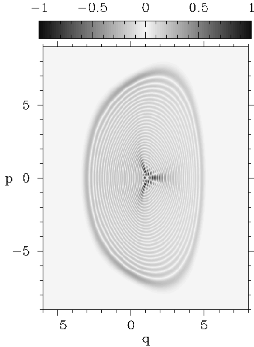
Fig. 9. Typical fringes for a semiclassical Wigner function. The classical curve follows closely the border of the fringes. The triangular structure of interfering fringes near the centre results from the unfolding of the maximum of the Fock states due to symmetry breaking.
