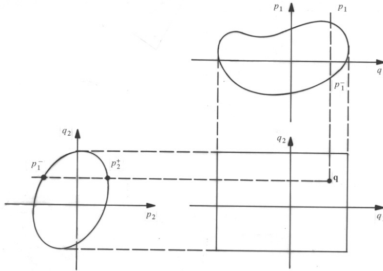
Fig. 3. Each point within the rectangular caustic of a two-dimensional product torus is the image of four phase space points under p -projection.
