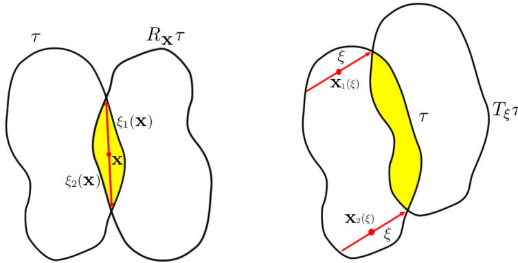
Fig. 8. (a) The semiclassical Wigner function is constructed by reflecting the torus \tau around the point \mathbf{x} : The chords \xi(\mathbf{x}) are defined by the intersections with R_{\mathbf{x}}\tau . (b) The semiclassical chord function is constructed by translating \tau by the vector \xi : The centres \mathbf{x}(\xi) lie halfway back along \xi from each intersection of \tau with T_{\xi}\tau .
