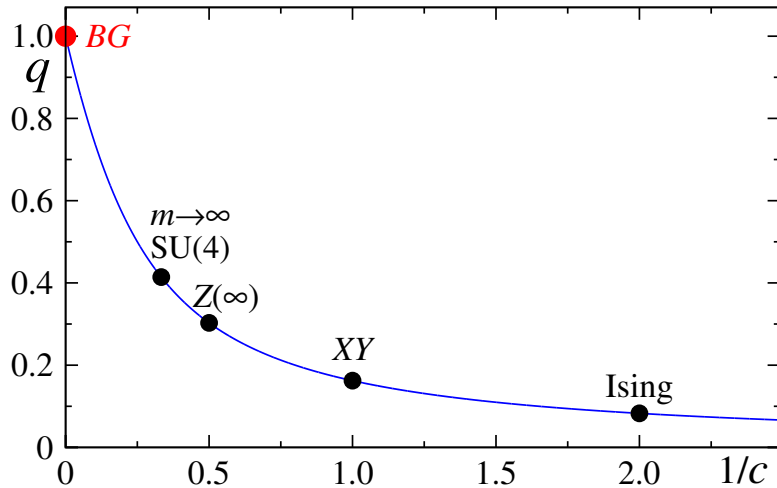
Fig. 2. The index q has been determined [30] from first principles, namely from the universality class of the Hamiltonian, characterized by the central charge c . The values c = 1/2 and c = 1 respectively correspond to the Ising and XY ferromagnetic chains in the presence of transverse field at T = 0 criticality. For other models see [32, 33]. In the c \rightarrow \infty limit we recover the Boltzmann-Gibbs (BG) value, i.e., q = 1 . For arbitrary value of c , the subsystem nonadditive entropy S_q is thermodynamically extensive for, and only for, q = \frac{\sqrt{9+c^2}-3}{c} .
