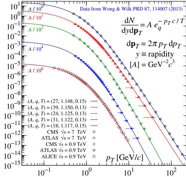
Fig. 3. Experimental distributions of the transverse moments in hadronic jets at the CMS, ALICE and ATLAS detectors at LHC. The data are from [103]. They can be remarkably well fitted (along fourteen decades) with the q -exponential function e_q^x \equiv [1 + (1 - q)x]^{1/(1-q)} , which, under appropriate constraints, extremizes the entropy S_q . See details in [104].
