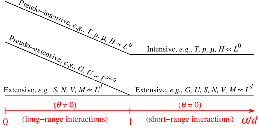
Fig. 1. Representation of the different scaling regimes of the Eq. (16) for classical d -dimensional systems. For attractive long-range interactions ( i.e. , 0 \leq \alpha/d \leq 1 , \alpha characterizes the interaction range in a potential with the form 1/r^\alpha ) we may distinguish three classes of thermodynamic variables, namely, those scaling with L^\theta , named pseudo-intensive ( L is a characteristic linear length, \theta is a system-dependent parameter), those scaling with L^{d+\theta} , the pseudo-extensive ones (the energies), and those scaling with L^d (which are always extensive). For short-range interactions ( i.e. , \alpha > d ) we have \theta = 0 and the energies recover their standard L^d extensive scaling, falling in the same class of S , N , V , etc, whereas the previous pseudo-intensive variables become truly intensive ones (independent of L ); this is the region, with two classes of variables, that is covered by the traditional textbooks of thermodynamics. From [10].
