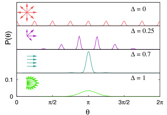
FIG. 4 (color online). Angle distribution for the four phases along the fixed temperature line T = 0.16 of the q = 8 phase diagram. All graphs have the same vertical scale.
