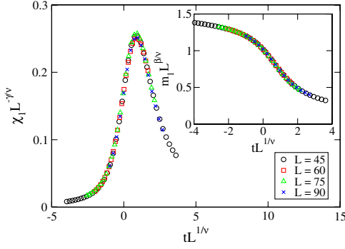
FIG. 2 (color online). Ferromagnetic-nematic transition for q = 3 . FSS analysis of the susceptibility \chi_1 and the order parameter m_1 (inset) for \Delta = 0.25 and different sizes L . In both cases the data collapse is excellent using the 3-state Potts exponents. The critical temperature at this point is T_c \approx 0.365 .
