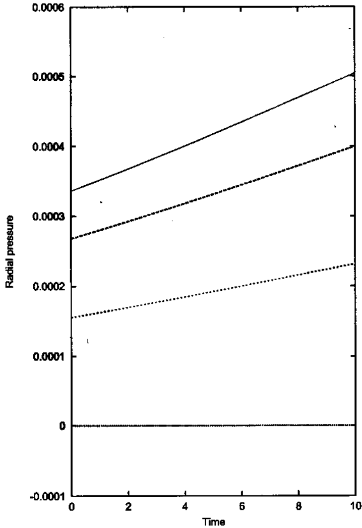
FIG. 2. Radial pressure, P_r m(0)^2 , as a function of time for the Schwarzschild-type model. The initial conditions are: A(0) = 5 , F(0) = 0.6 and \Omega(0) = -0.1 . Curves represent different regions: r/r_\Sigma = 0.25 (continuous line); 0.50 (dashed line); 0.75 (short-dashed line) and 1.00 (dotted line).
