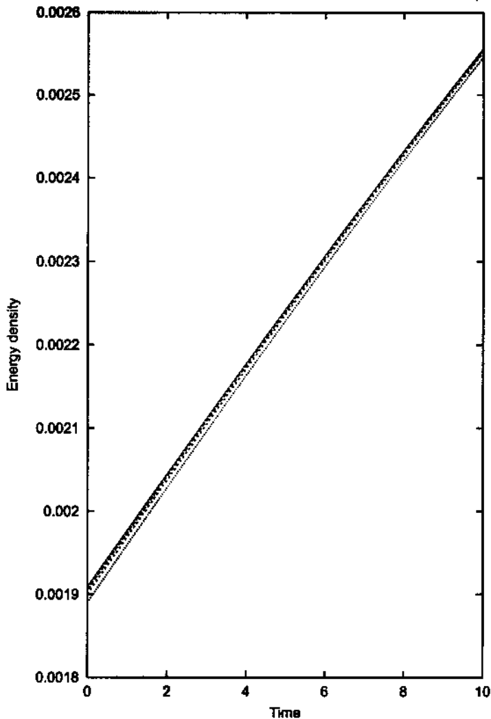
FIG. 1. Energy density, \rho m(0)^2 , as a function of (dimensionless) time ( \alpha ) for the Schwarzschild-type model. The initial conditions are: A(0) = 5 , F(0) = 0.6 and \Omega(0) = -0.1 . Curves represent different regions: r/r_\Sigma = 0.25 (continuous line); 0.50 (dashed line); 0.75 (short-dashed line) and 1.00 (dotted line).
