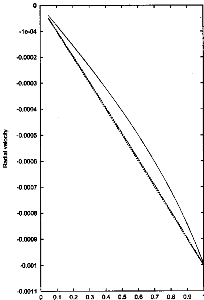
FIG. 6. Radial velocity, \omega , as a function of r/r_\Sigma for \alpha = 10 . The initial velocity at the surface is -0.001 . Curves represent different values of F(0) : 0.6 (continuous line); 0.96 (dashed line) and 0.996 (short-dashed line).
