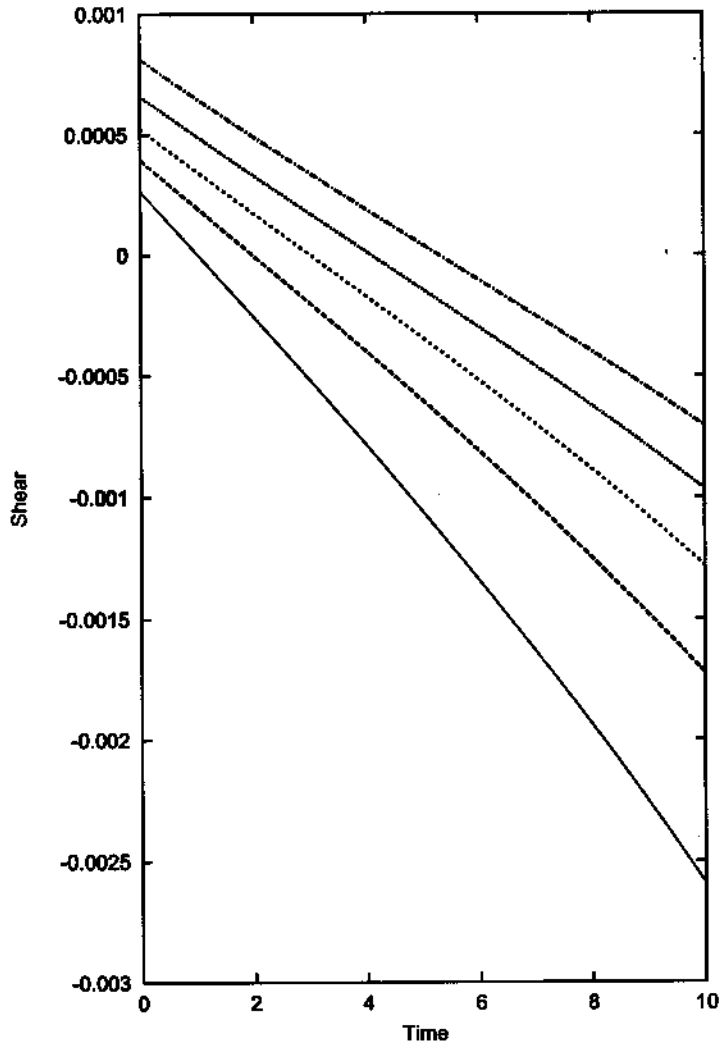
FIG. 11. Shear, \sigma m(0) , as a function of time for the Tolman VI-type model. The initial conditions are: F(0) = 0.581428528 and \Omega(0) = -0.0001 . Curves represent different regions: r/r_\Sigma = 0.2 (continuous line); 0.4 (dashed line); 0.6 (short-dashed line); 0.8 (dotted line) and 1.0 (dot-dashed line).
