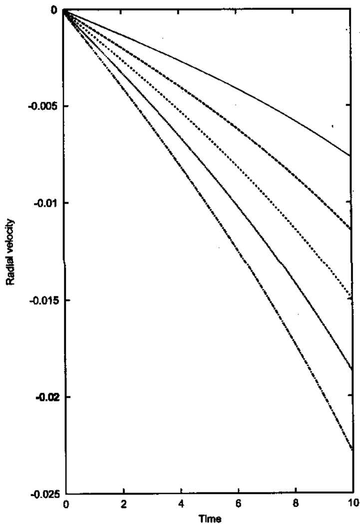
FIG. 8. Radial velocity, \omega , as a function of time for the Tolman-type model. The initial conditions are: F(0) = 0.561428547 and \Omega(0) = -0.0001 . Curves represent different regions: r/r_\Sigma = 0.2 (continuous line); 0.4 (dashed line); 0.6 (short-dashed line); 0.8 (dotted line) and 1.0 (dot-dashed line).
