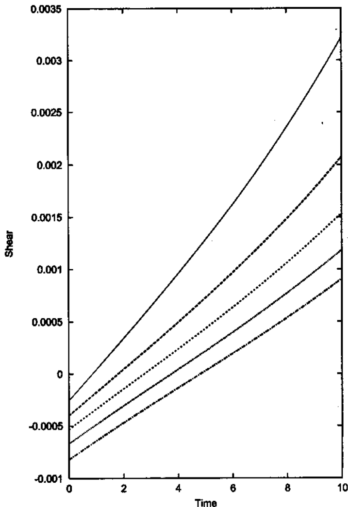
FIG. 12. Shear, \sigma m(0) , as a function of time for the Tolman-type model. The initial conditions are: F(0) = 0.561428547 and \Omega(0) = -0.0001 . Curves represent different regions: r/r_{\Sigma} = 0.2 (continuous line); 0.4 (dashed line); 0.6 (short-dashed line); 0.8 (dotted line) and 1.0 (dot-dashed line).
