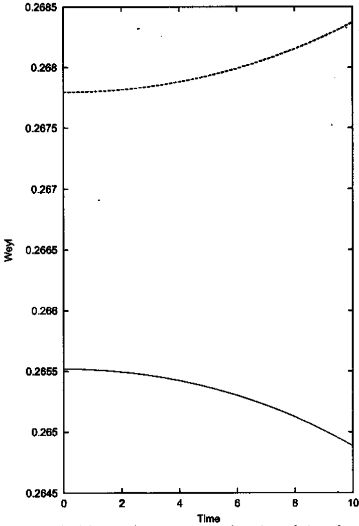
FIG. 9. Weyl tensor, W/m(0) , at r/r_{\Sigma} = 0.4 as a function of time for the Tolman VI-type model. The initial conditions are: F(0) = 0.581428528 (dashed line); F(0) = 0.561428547 (continuous line) and \Omega(0) = -0.0001 .
