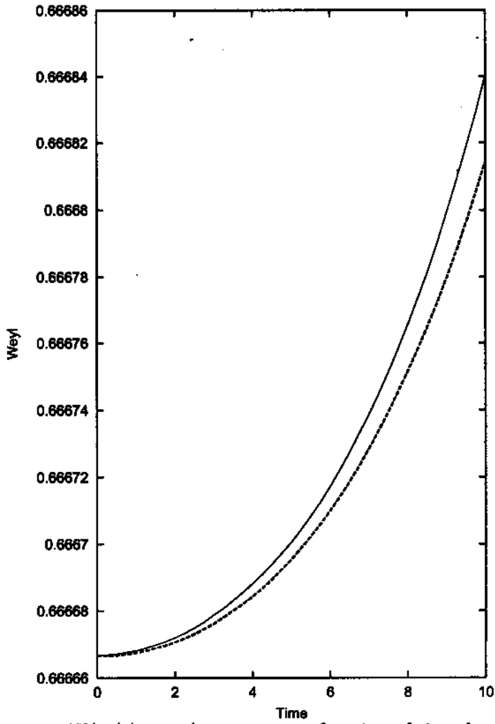
FIG. 10. Weyl tensor, W/m(0) , at r/r_{\Sigma} = 1.0 as a function of time for the Tolman VI-type model. The initial conditions are: F(0) = 0.581428528 (dashed line); F(0) = 0.561428547 (continuous line) and \Omega(0) = -0.0001 .
