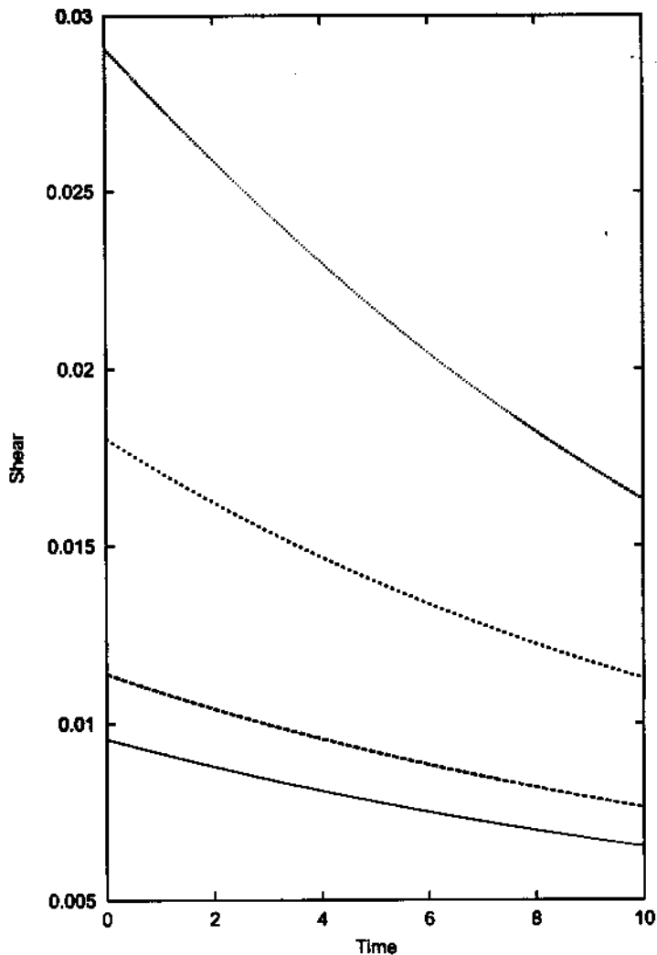
FIG. 4. Shear, \sigma m(0) , as a function of time for the Schwarzschild-type model. The initial conditions are: A(0) = 5 , F(0) = 0.6 and \Omega(0) = -0.1 . Curves represent different regions: r/r_{\Sigma} = 0.25 (continuous line); 0.50 (dashed line); 0.75 (short-dashed line) and 1.00 (dotted line).
