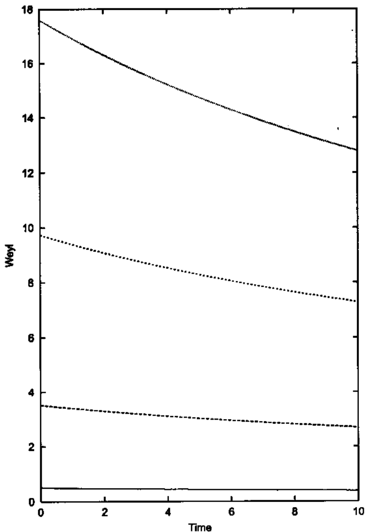
FIG. 5. Weyl tensor, W/m(0) , as a function of time for the Schwarzschild-type model. The initial conditions are: A(0) = 5 , F(0) = 0.6 and \Omega(0) = -0.1 . Curves represent different regions: r/r_\Sigma = 0.25 (continuous line); 0.50 (dashed line); 0.75 (short-dashed line) and 1.00 (dotted line).
