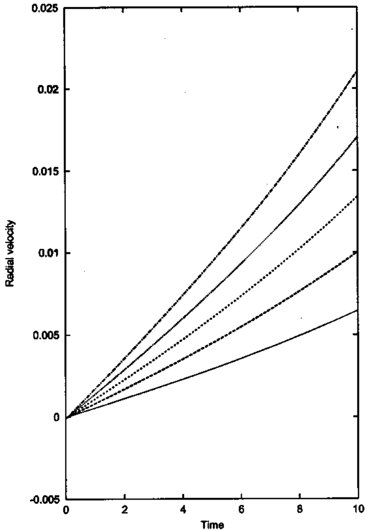
FIG. 7. Radial velocity, \omega , as a function of time for the Tolman VI-type model. The initial conditions are: F(0) = 0.581428528 and \Omega(0) = -0.0001 . Curves represent different regions: r/r_{\Sigma} = 0.2 (continuous line); 0.4 (dashed line); 0.6 (short-dashed line); 0.8 (dotted line) and 1.0 (dot-dashed line).
