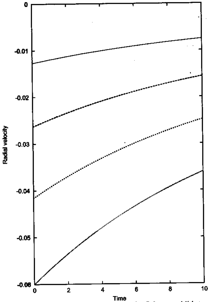
FIG. 3. Radial velocity, \omega , as a function of time for the Schwarzschild-type model. The initial conditions are: A(0) = 5 , F(0) = 0.6 and \Omega(0) = -0.1 . Curves represent different regions: r/r_\Sigma = 0.25 (continuous line); 0.50 (dashed line); 0.75 (short-dashed line) and 1.00 (dotted line).
