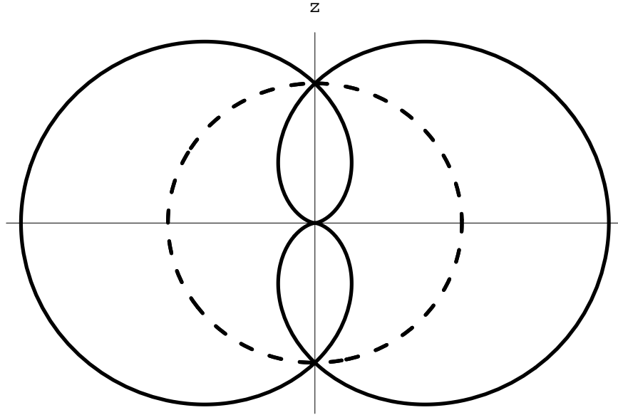
Figure 4: Ergospheres (with solid lines) and horizons (with dashed lines) of a extreme DN black-hole for the following values, a = M = 4 , of the parameters. We plot here the intersections of the plane \phi = cte with the surfaces of revolution, obtained from the rotation of these curves around the z axis. Notice the continuity of the two ergospheres and of their slopes. The two horizons are the same, r_{\pm} = M = 4 .
