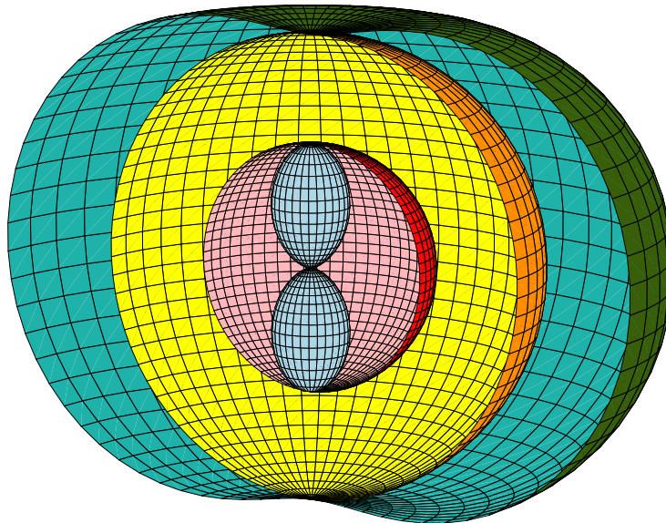
Figure 5: Ergospheres and horizons of DN spacetime for the following values, a = 4 and M = 4.2 , of the parameters.
