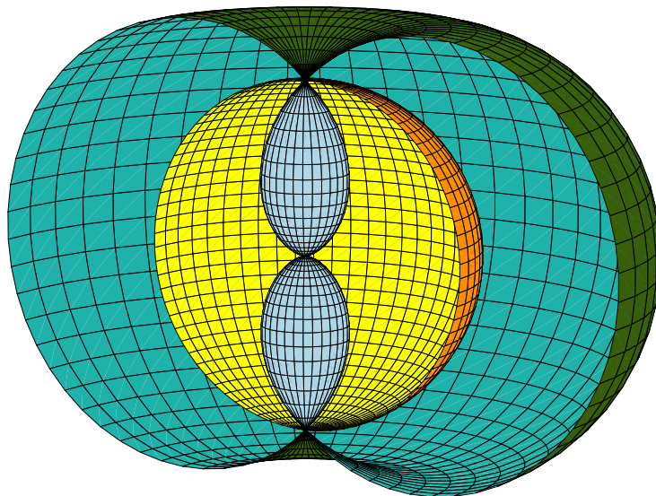
Figure 6: Ergospheres and horizons of a extreme DN black-hole for the following values, a = M = 4 , of the parameters.
