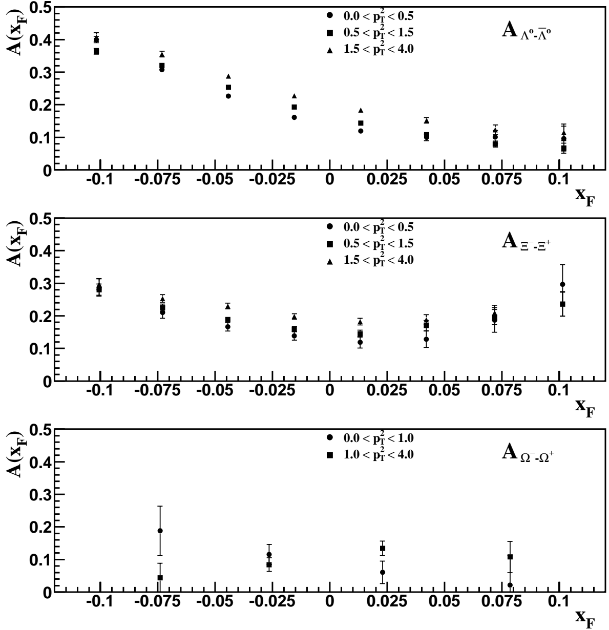
Figure 3.: \Lambda^0 - \bar{\Lambda}^0 (upper), \Xi^- - \Xi^+ (middle), and \Omega^- - \Omega^+ (lower) production asymmetries as a function of x_F in different p_T^2 regions.
