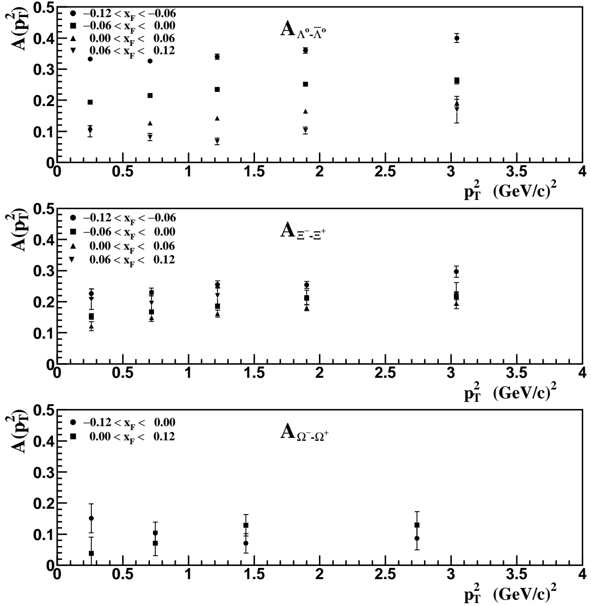
Figure 4.: \Lambda^0 - \bar{\Lambda}^0 (upper), \Xi^- - \Xi^+ (middle), and \Omega^- - \Omega^+ (lower) production asymmetries as a function of p_T^2 in different x_F regions.
