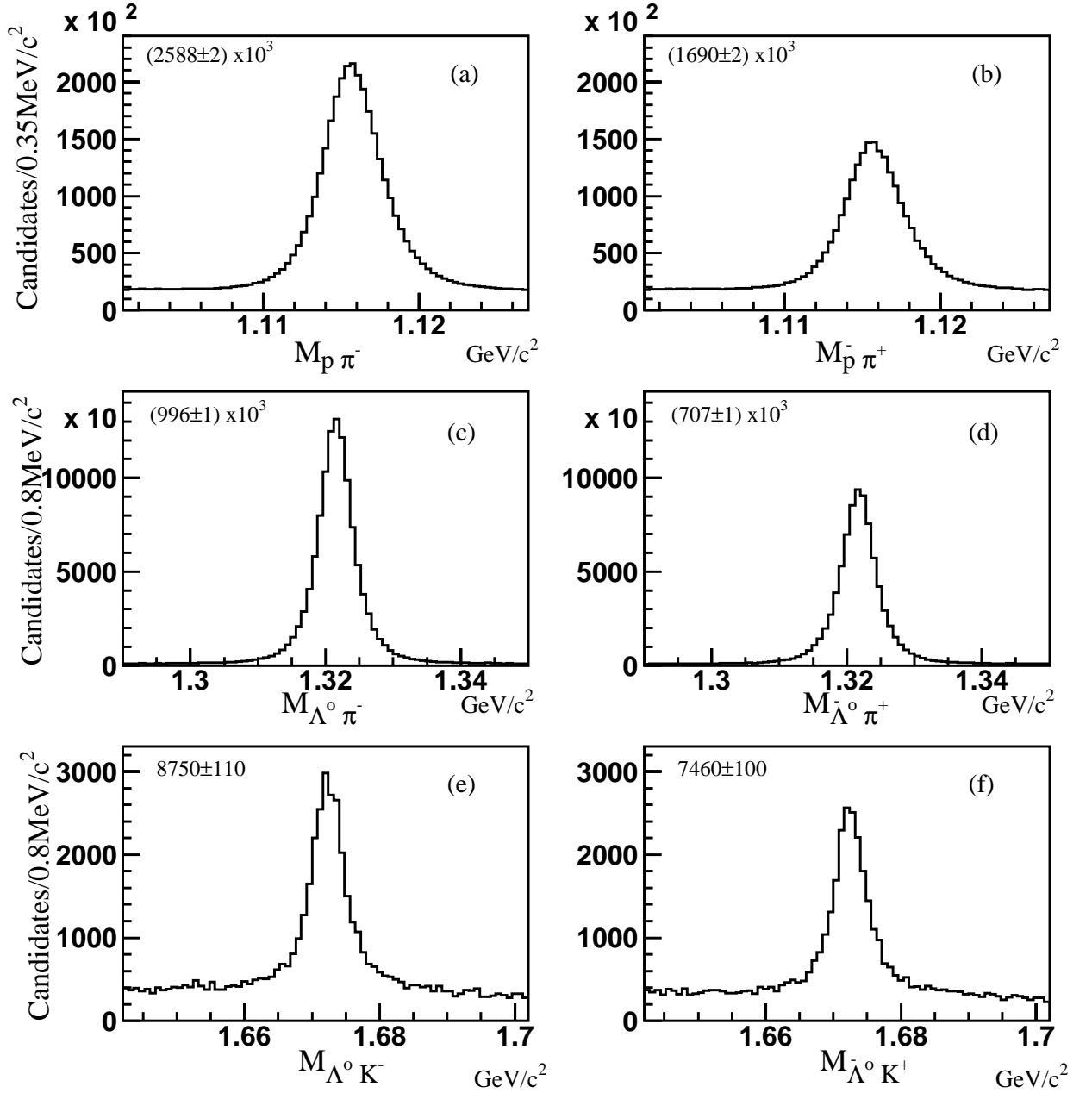
Figure 1.: Effective mass distributions for decay products of hyperons in events selected for this study and the corresponding signals with background subtracted. Plots correspond to (a) \Lambda^0 \rightarrow p\pi^- ; (b) \bar{\Lambda}^0 \rightarrow \bar{p}\pi^+ ; (c) \Xi^- \rightarrow \Lambda^0\pi^- ; (d) \Xi^+ \rightarrow \bar{\Lambda}^0\pi^+ ; (e) \Omega^- \rightarrow \Lambda^0 K^- (f) \Omega^+ \rightarrow \bar{\Lambda}^0 K^+ . The numbers and errors in the top corner of each plot come from the sum of the number of background subtracted events in the individual (x_F, p_T^2) bin fits.
