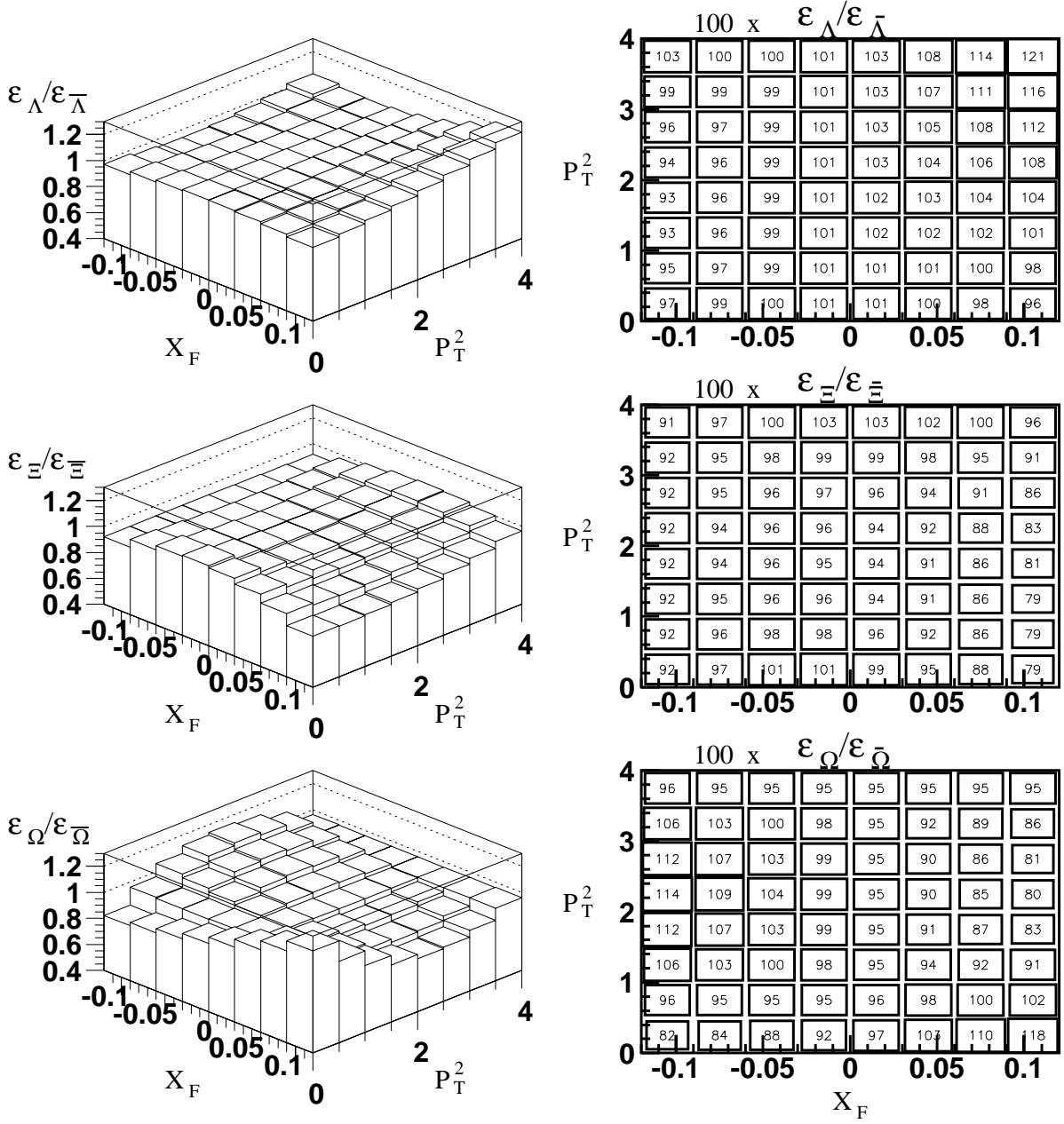
Figure 2.: Ratio of efficiencies as functions of x_F and p_T^2 for the three hyperons. The transverse momentum axes are in units of (\text{GeV}/c)^2 .
