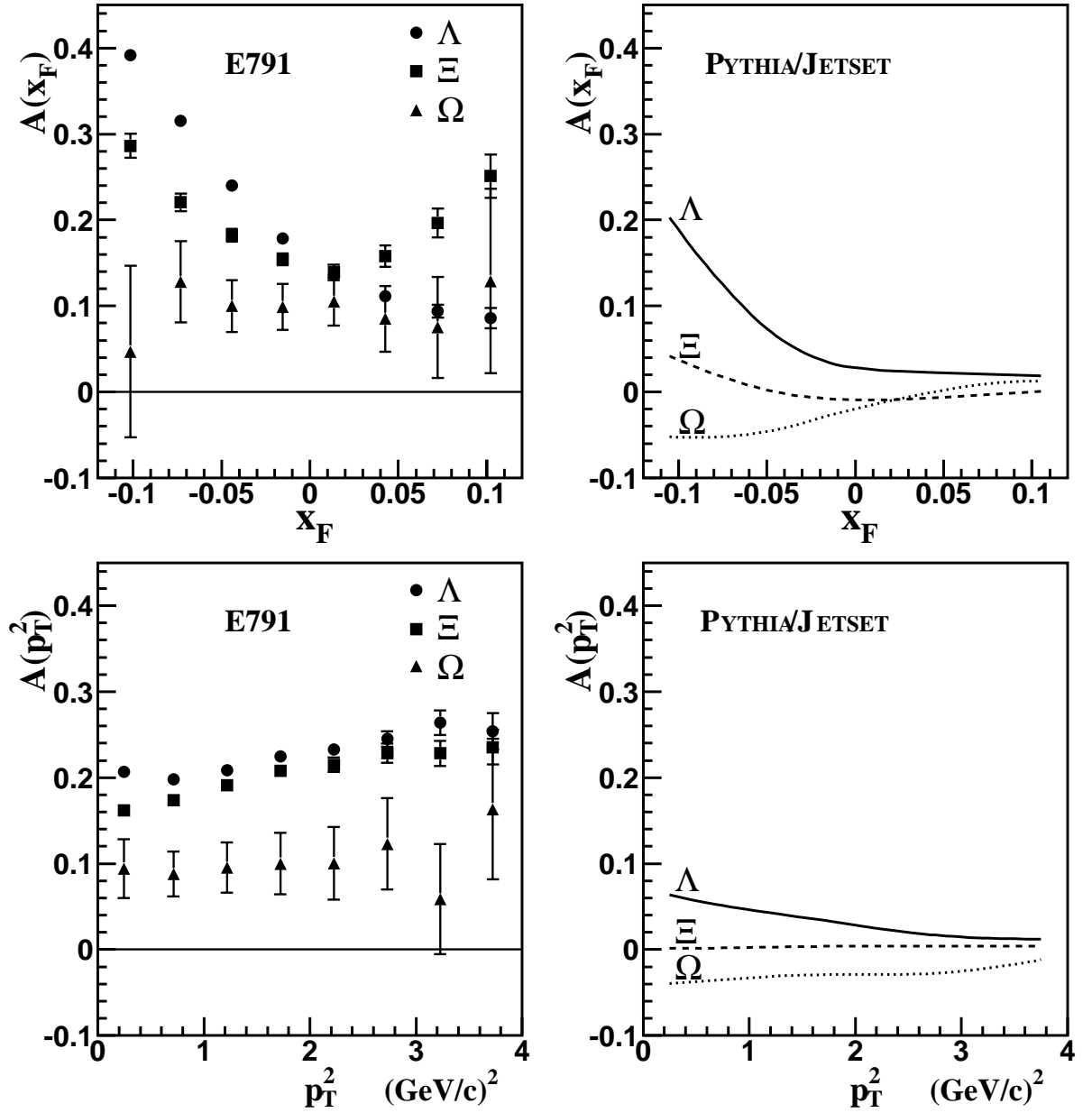
Figure 5.: Comparison among the asymmetries in the production of the three hyperons for the E791 data and PYTHIA/JETSET predictions. The error bars of the E791 data include the statistical and systematic uncertainties
