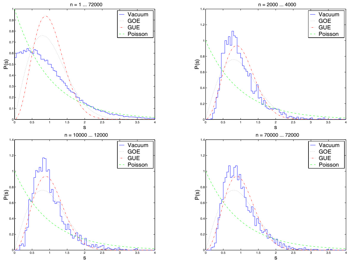
Figure 1: The statistical of level-spacings in vacuum spectra \{p_n t_n\} . The histogram at the top left gives a sequence comprising the first 72000 vacuum levels. The histogram at the top right comprises 2000 consecutive levels in the analysis corresponding from the 2000 th to the 4000 th level. The histograms at the bottom give 2000 consecutive levels centered at different E values.
