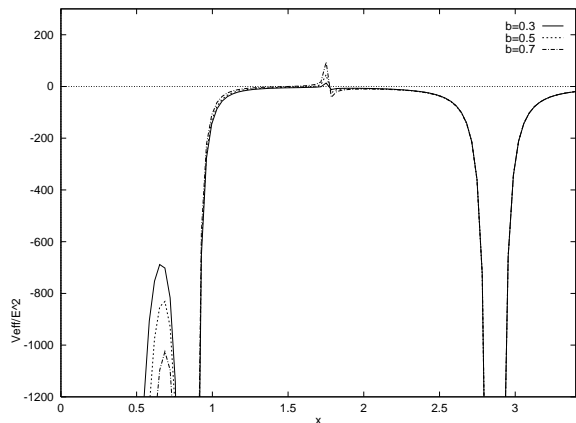
FIG. 4. Effective potential V_{\text{eff}}/E_0^2 for s = 4 and different values of b . The interval 1.7 \leq x \leq 1.8 is shown in detail in the next figure.
