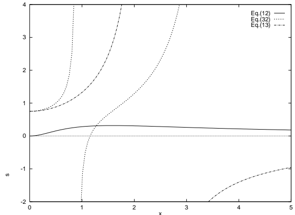
FIG. 6. Position of the zeros of the metric and spacetime singularities for a given s .
