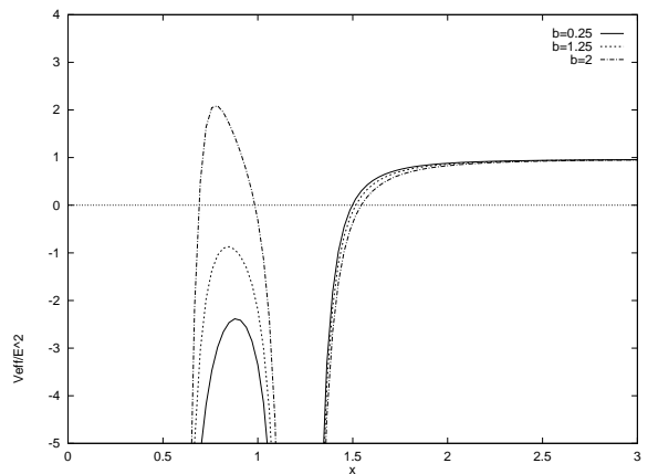
FIG. 3. Effective potential V_{\text{eff}}/E_0^2 for s = 0.2 and different values of the impact parameter b = h_0/E_0 .
