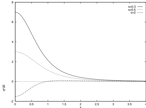
FIG. 2. Energy density of the electric field times q^2 as a function of x for different values of s .
