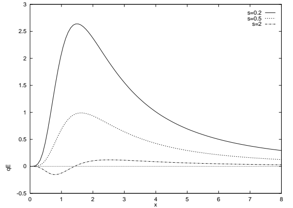
FIG. 1. Electric field times the electric charge q as a function of x for different values of s .
