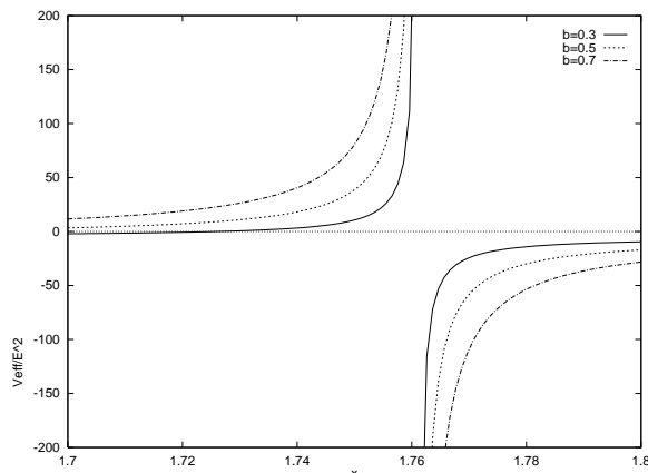
FIG. 5. Effective potential V_{\text{eff}}/E_0^2 for s = 4 and different values of b . The singularity seen in this plot comes from the pole of \mathcal{L}_F .
