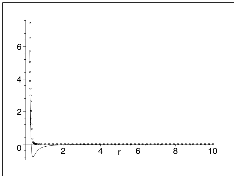
Figure 1: Plot of the pure MCS potential (box dotted line) \times plot of the gauge potential (continuous line) for the following parameter values: s = 20 , v = 5 , \beta = \pi/2 , m_e = 5.10^5 .
