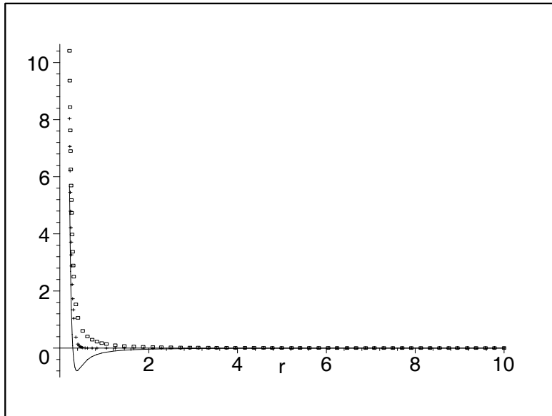
Figure 3: Plot of the gauge potential for s = 20, v = 5, m = 5 \cdot 10^5 and \beta = \pi/2 (continuous line), \beta = 3\pi/4 (box dotted line), \beta = \pi (cross dotted line).
