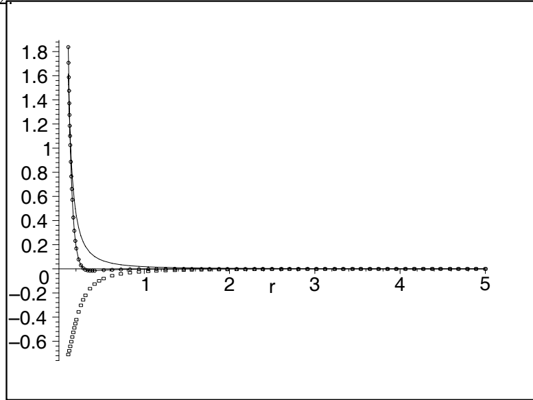
Figure 2: Plot of the gauge potential (dotted line) \times effective potential (continuous line) for two set of parameters with distinct mass value: (s = 20, v = 5, m = 50, \beta = \pi/2, L = 1) and (s = 20, v = 5, m = 5.10^5, \beta = \pi/2, L = 1) .
