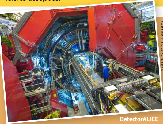
Detector ALICE
