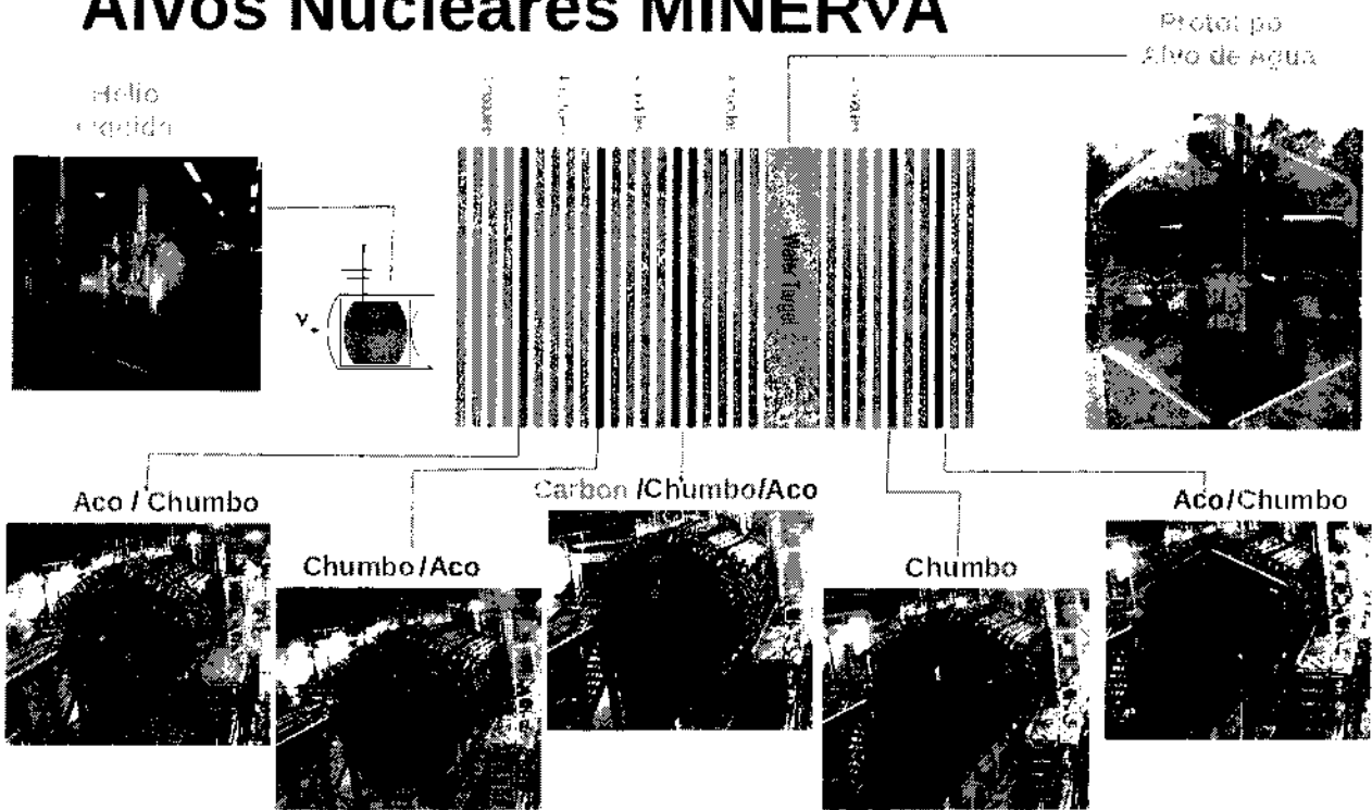
Figure 3.11: MINERvA Nuclear targets
