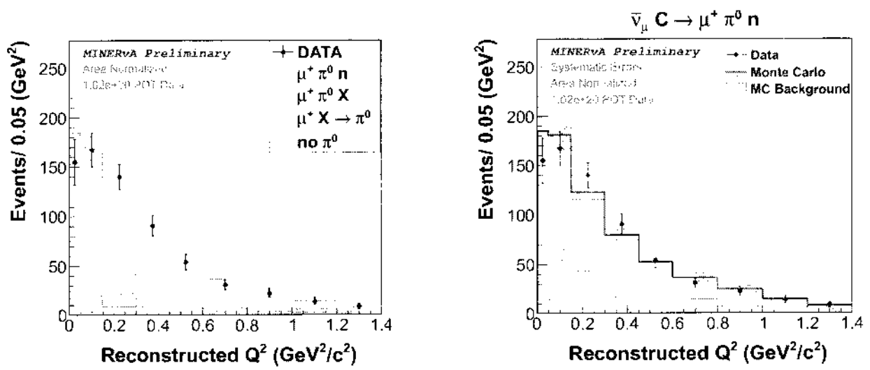
Figure 5.37: Left: Q^2 for CC\pi^0 inclusive, data and Monte Carlo, relative normalize, stack plot. Right: Q^2 for CC\pi^0 exclusive including Monte Carlo background.
