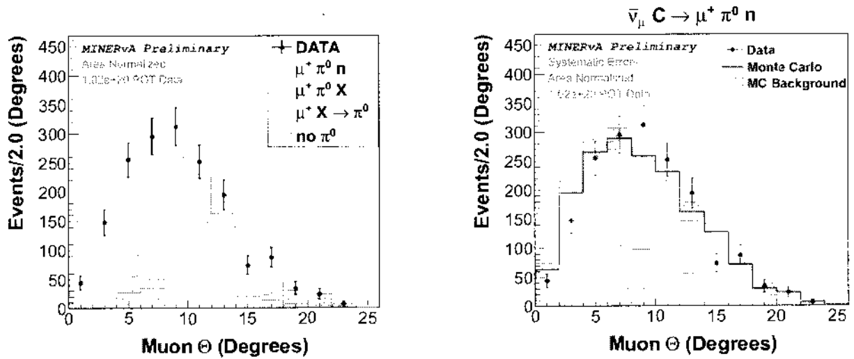
Figure 5.34: Left: \theta angle of the muon direction, data and Monte Carlo, stack plot. Right: \theta angle of the muon direction including Monte Carlo Background for CC\pi^0 exclusive
