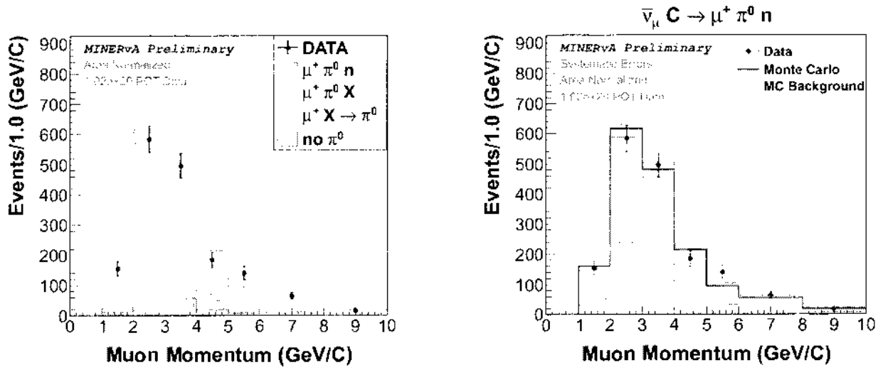
Figure 5.33: Left: muon momentum, data and Monte Carlo, stack plot for CC\pi^0 exclusive. Right: muon momentum including Monte Carlo background.
