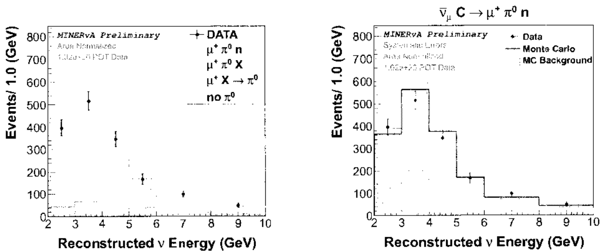
Figure 5.36: Left: E_{\nu_\mu} for CC\pi^0 inclusive, data and Monte Carlo, relative normalized, stack plot. Right: E_{\nu_\mu} for CC\pi^0 exclusive including Monte Carlo background.
