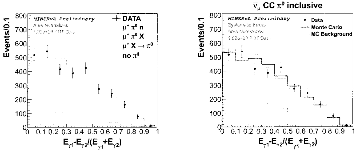
Figure 5.17: Left: (E_{\gamma_1} - E_{\gamma_2}) / (E_{\gamma_1} + E_{\gamma_2}) , data and Monte Carlo. Right: (E_{\gamma_1} - E_{\gamma_2}) / (E_{\gamma_1} + E_{\gamma_2}) , data and Monte Carlo. Monte Carlo Background for CC\pi^0 inclusive is included.
