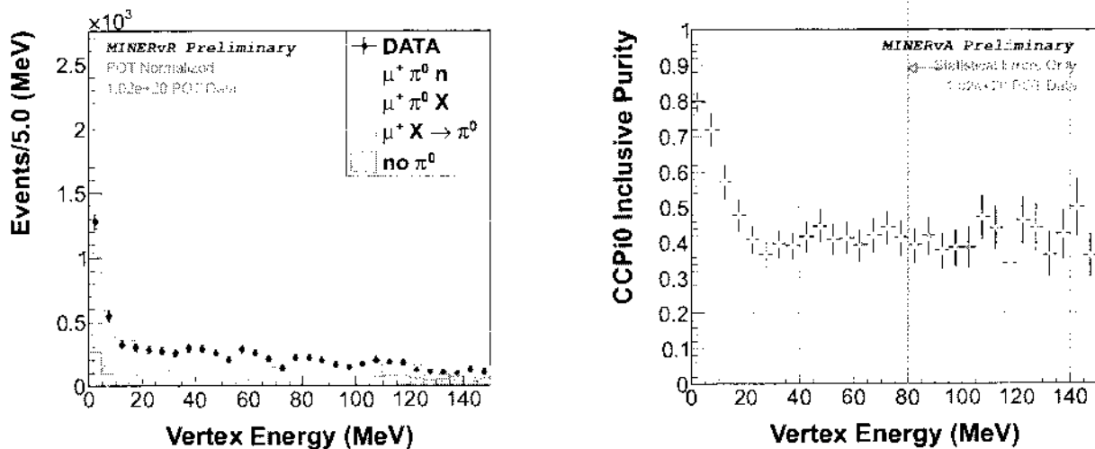
Figure 5.12: Left: Vertex Energy including our categories. Right: CC\pi^0 inclusive purity versus vertex energy dependence. We define a cut at vertex energy equals to 80\text{MeV}
