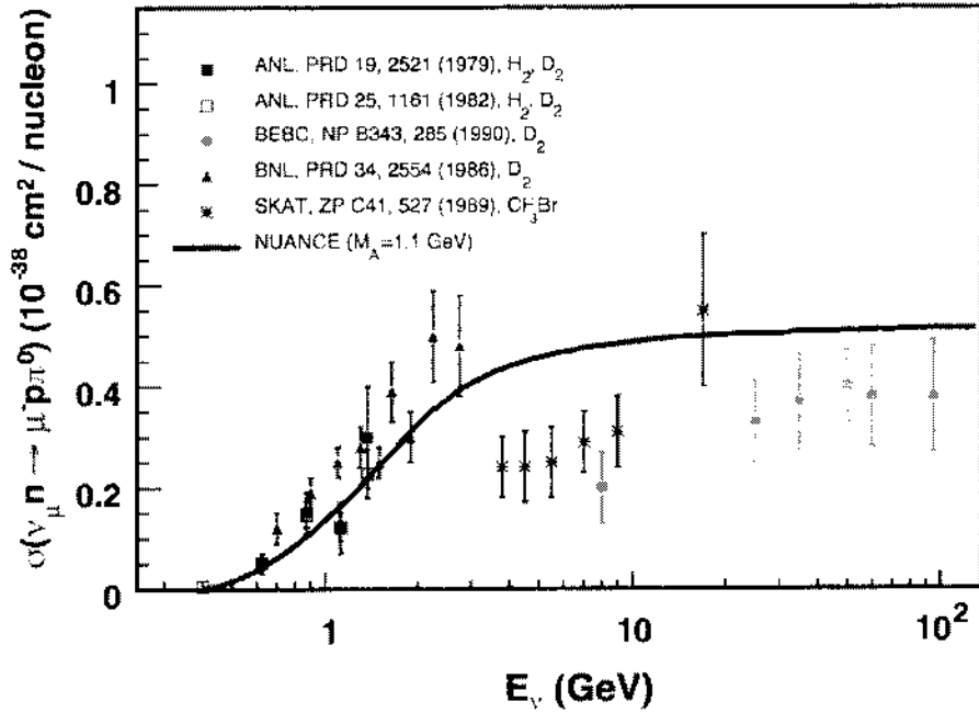
Figure 2.5: Current cross section measurements for the CC process, \nu_\mu n \rightarrow \mu^- p \pi^0 , as a function of neutrino energy.
