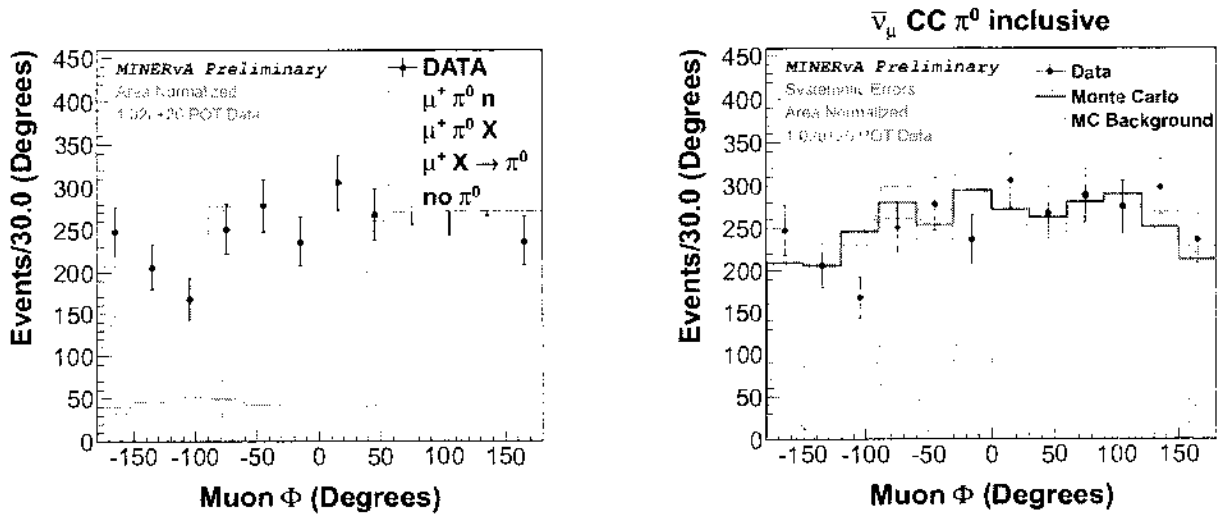
Figure 5.24: Left: \phi angle of the muon direction, data and Monte Carlo, stack plot. Right: \phi angle of the muon direction including Monte Carlo background for CC\pi^0 inclusive
