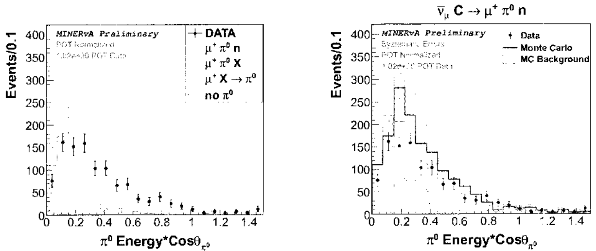
Figure 5.32: Left: E_{\pi^0} \times \cos\pi^0 , data and Monte Carlo, stack plot. Right: E_{\pi^0} \times \cos\pi^0 including Monte Carlo Background for CC\pi^0 exclusive.
