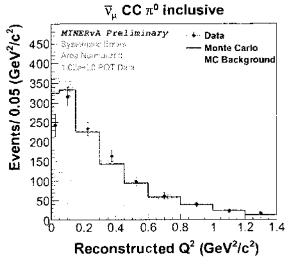
Figure 5.26: Left: Q^2 for CC\pi^0 inclusive, data and Monte Carlo, relative normalize, stack plot. Right: Q^2 for CC\pi^0 inclusive, including Monte Carlo Background
