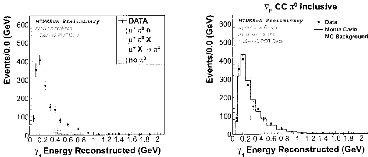
Figure 5.16: Left: \gamma_1 energy distribution, data and Monte Carlo. Stack plot includes all our categories. Right: \gamma_1 energy distribution, data and Monte Carlo (Monte Carlo background included).
