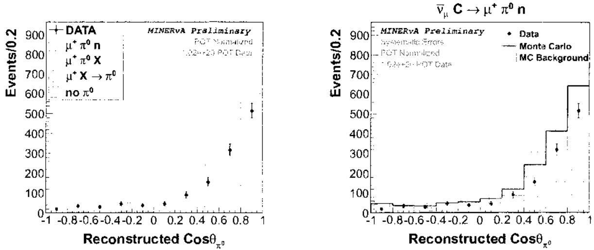
Figure 5.31: Left: Cosine opening angle between \pi^0 and \nu_\mu direction, data and Monte Carlo, stack plot for CC\pi^0 exclusive. Right: Cosine opening angle between \pi^0 and \bar{\nu}_\mu direction, including Monte Carlo background.
