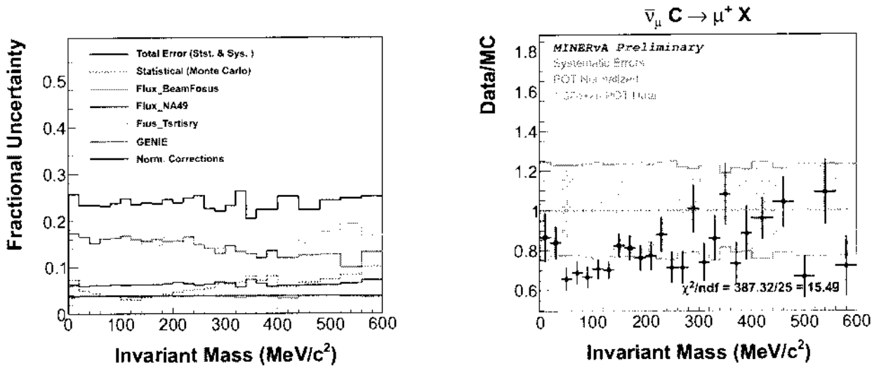
Figure 5.8: Left: Error summary plot for the invariant mass, where Y axis is fractional uncertainty. Right: Ratio between data and reconstructed Monte Carlo (sidebands are the systematic errors).
