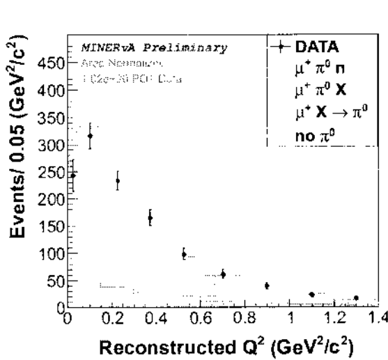
Figure 5.26: Left: Q^2 for CC\pi^0 inclusive, data and Monte Carlo, relative normalize, stack plot. Right: Q^2 for CC\pi^0 inclusive, including Monte Carlo Background
