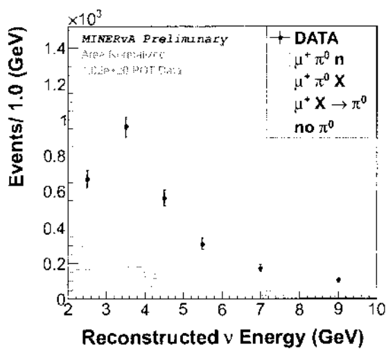
Figure 5.25: Left: E_{\bar{\nu}_\mu} for CC\pi^0 inclusive, data and Monte Carlo, relative normalize, stack plot. Right: E_{\bar{\nu}_\mu} for CC\pi^0 inclusive including Monte Carlo background.
