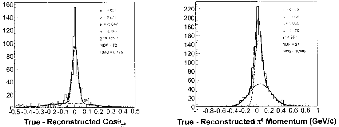
Figure B.1: Left: \cos\theta_{\pi^0} residuals for CC\pi^0 exclusive events. Right: \pi^0 momentum residuals for CC\pi^0 exclusive sample.
