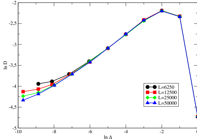
FIG. 2: (Color online) Asymptotic diffusion rate versus \Delta in model II.
