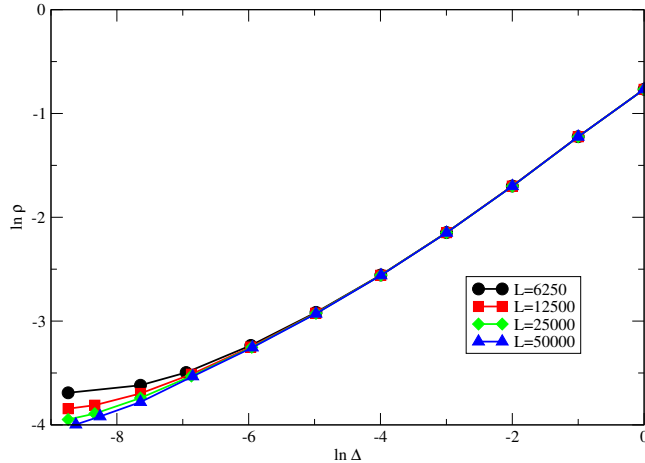
FIG. 3: (Color online) Stationary activity density \rho versus \Delta in model I.
