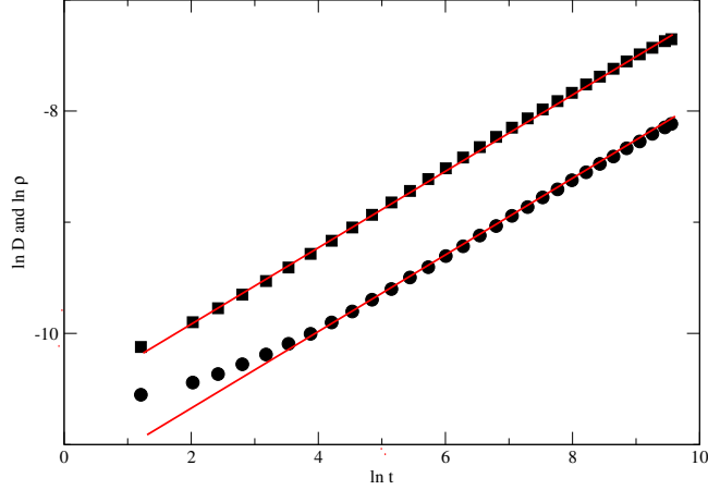
FIG. 8: (Color online) Initial growth of activity (squares) and diffusion rate (circles) at criticality in model II, starting with a single active site; system size L = 50\,000 .
