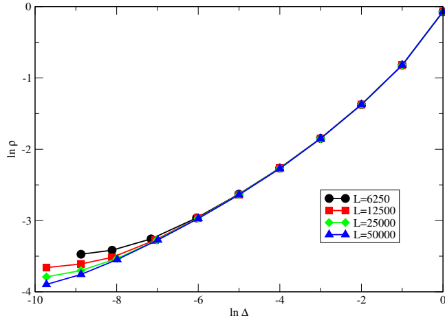
FIG. 4: (Color online) Stationary activity versus \Delta in model II.
