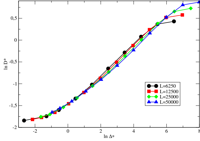
FIG. 6: (Color online) Scaled diffusion rate D^* = L^{\beta/\nu_{\perp}} D versus scaled distance from critical point \Delta^* = L^{1/\nu_{\perp}} \Delta in model I.
