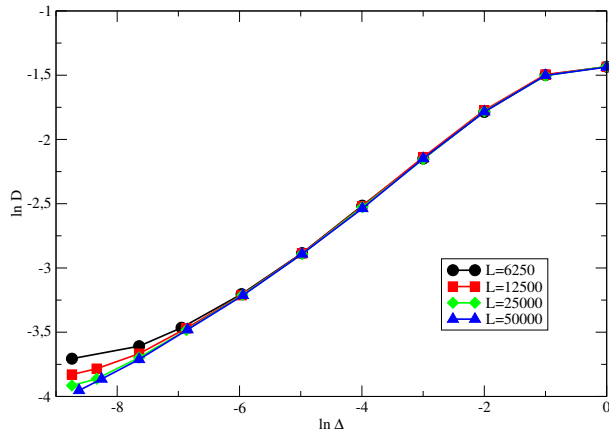
FIG. 1: (Color online) Asymptotic diffusion rate versus \Delta = p - p_c in model I, system sizes as indicated. Error bars are smaller than the symbols.
