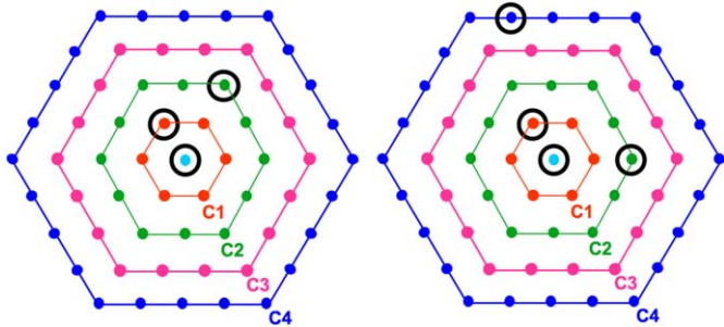
Fig. 2. Example of T3 configurations: the 3-fold T3 mode ToT2C_1&3C_2 is shown on the left and the 4-fold mode 2C_1&3C_2&4C_4 on the right (see text for the definitions). C_1 , C_2 , C_3 , C_4 indicate the first, second, third and fourth sets of neighbours, respectively, at 1.5, 3, 4.5 and 6 km from a given detector.
